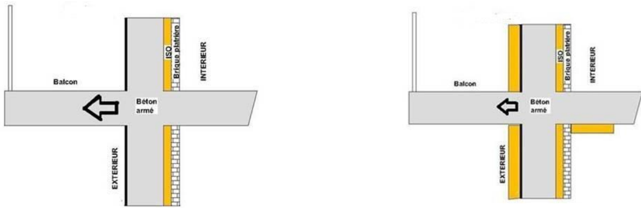
Figure 7 The PB of Building Insulation
