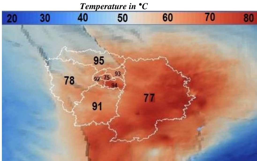
BRGM map of dogger geothermal water temperatures at a depth of between 1800 and 2000 m
